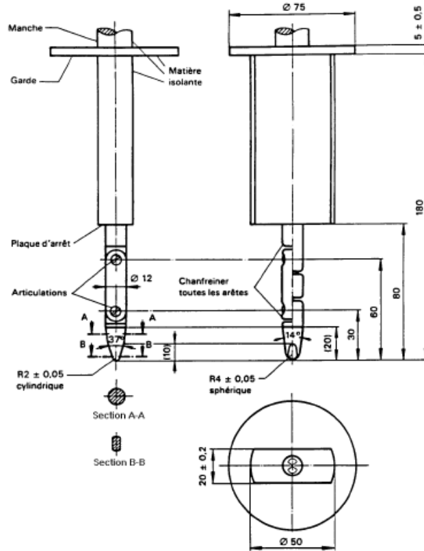
Figure n°1 : Test Probe B (jointed finger probe)
